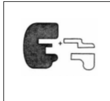
Enzyme + products
